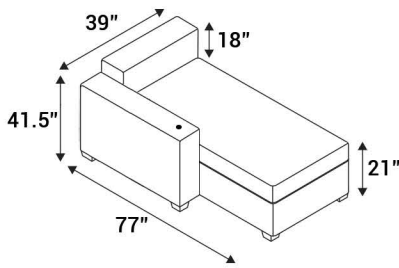
LAF Chaiselounger
