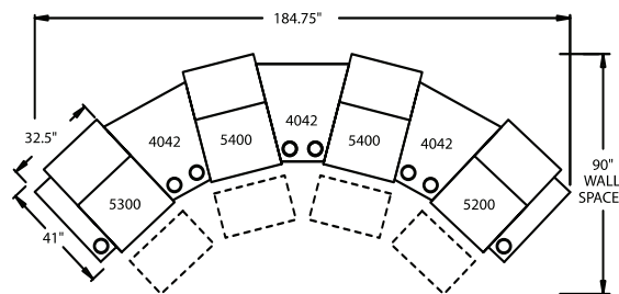
4 Seat Curved w/Wedge Console
