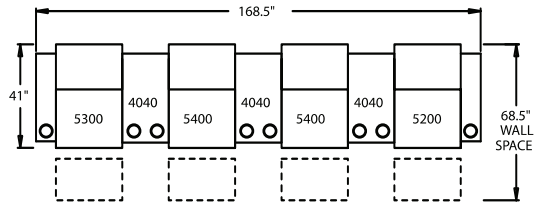
4 Seat Straight w/Straight Console
