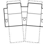
2 Seats Curved Configuration 71 x 69" 180 x 175cm
